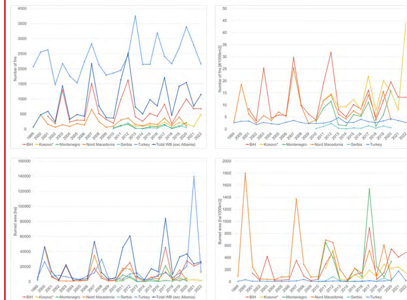
Figure 2: Shows the number of fires and burnt areas in the Western Balkans and Türkiye. On the top left, the total number of fires is reported while on bottom left the total burnt area is shown. On the top right, the number of fires over 1,000 km 2 is shown, while the bottom right indicates the burnt area over 1,000 km 2 .
